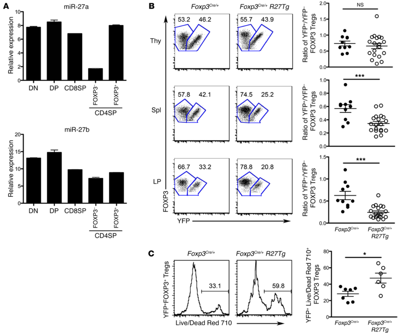
Figure 4. Optimal miR-27 expression is required to maintain normal Treg development and homeostasis. (A) qPCR analysis of miR-27a/b expression in different thymocyte subsets. Data represent the mean ± SD and are representative of 3 independent experiments (n = 3–6). (B) FACS analysis and ratios of YFP-Cre + and YFP-Cre - cells within the FOXP3 + CD4 + T cell population from FOXP3 Cre/+ R27Tg mice and FOXP3 Cre/+ control females. FACS data represent 4 independent experiments. (C) Viability of YFP-Cre + Tregs from the indicated mice was measured by Live/Dead staining after in vitro stimulation with plate-bound anti-CD3 and anti-CD28 for 6 hours. FACS data represent 3 independent experiments. Each symbol represents an individual mouse, and the bar represents the mean. *P < 0.05 and ***P < 0.001. P values are determined by an unpaired, 2-tailed Student's t test.
